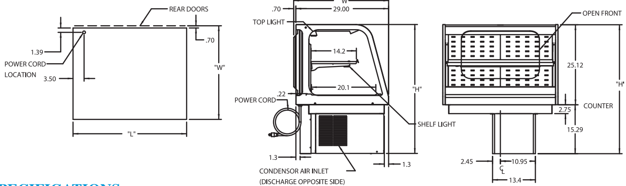
BOTTOM MOUNT
