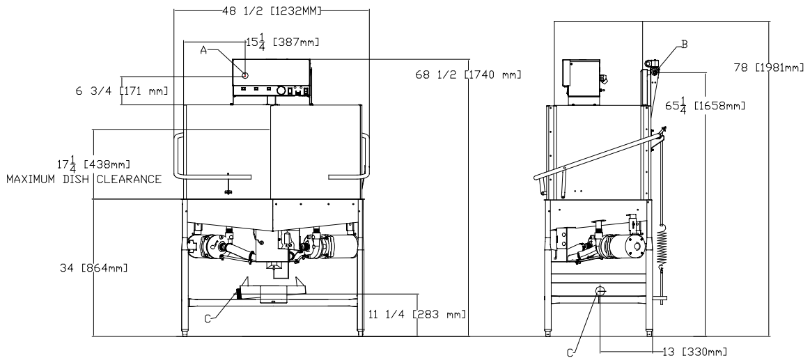
DIMENSIONS--INCHES (mm)--STANDARD MODEL
