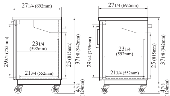
TBB-3SBD-N6 & TBB-3SGD-N SIDE VIEW
