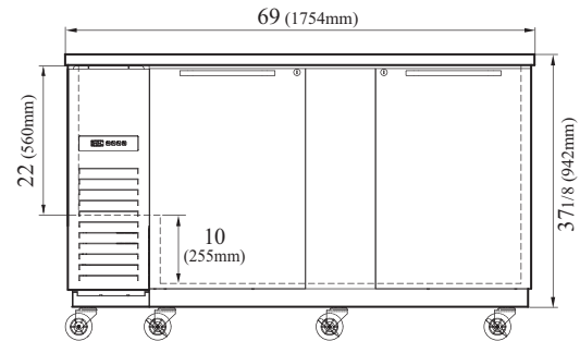
TBB-3SBD-N6 FRONT VIEW
