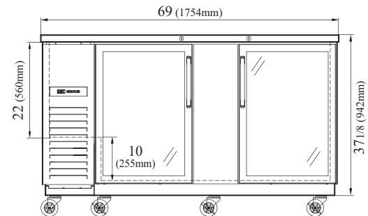
TBB-3SGD-N FRONT VIEW
