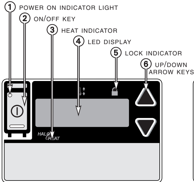
Electronic Control
